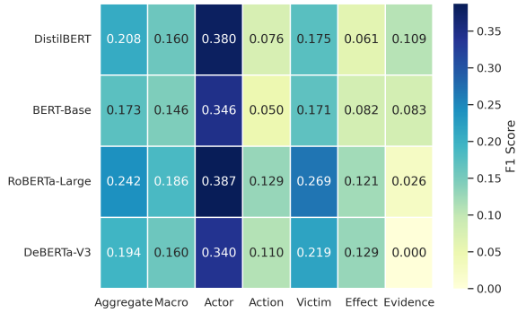
Figure 5: Performance Heatmap of Conspiracy Marker Extraction.
